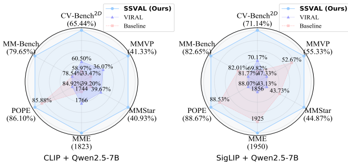
(a) Benchmark Performance
