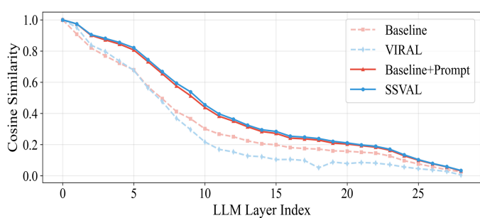
(b) Layer-wise Cosine Similarity to Input
